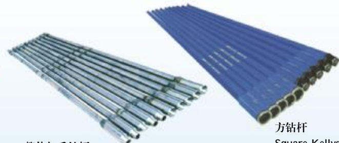
整体加重钻杆 Integral heavy weight drill pipes
