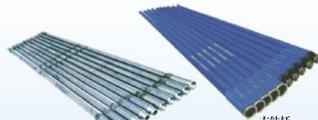
整体加重钻杆 Integral heavy weight drill pipes
